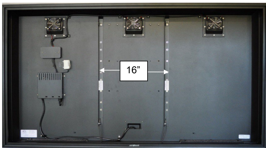
Picture illustrates 65" Apollo Enclosure with brackets in 400mm position. (Approximately 16" apart.
